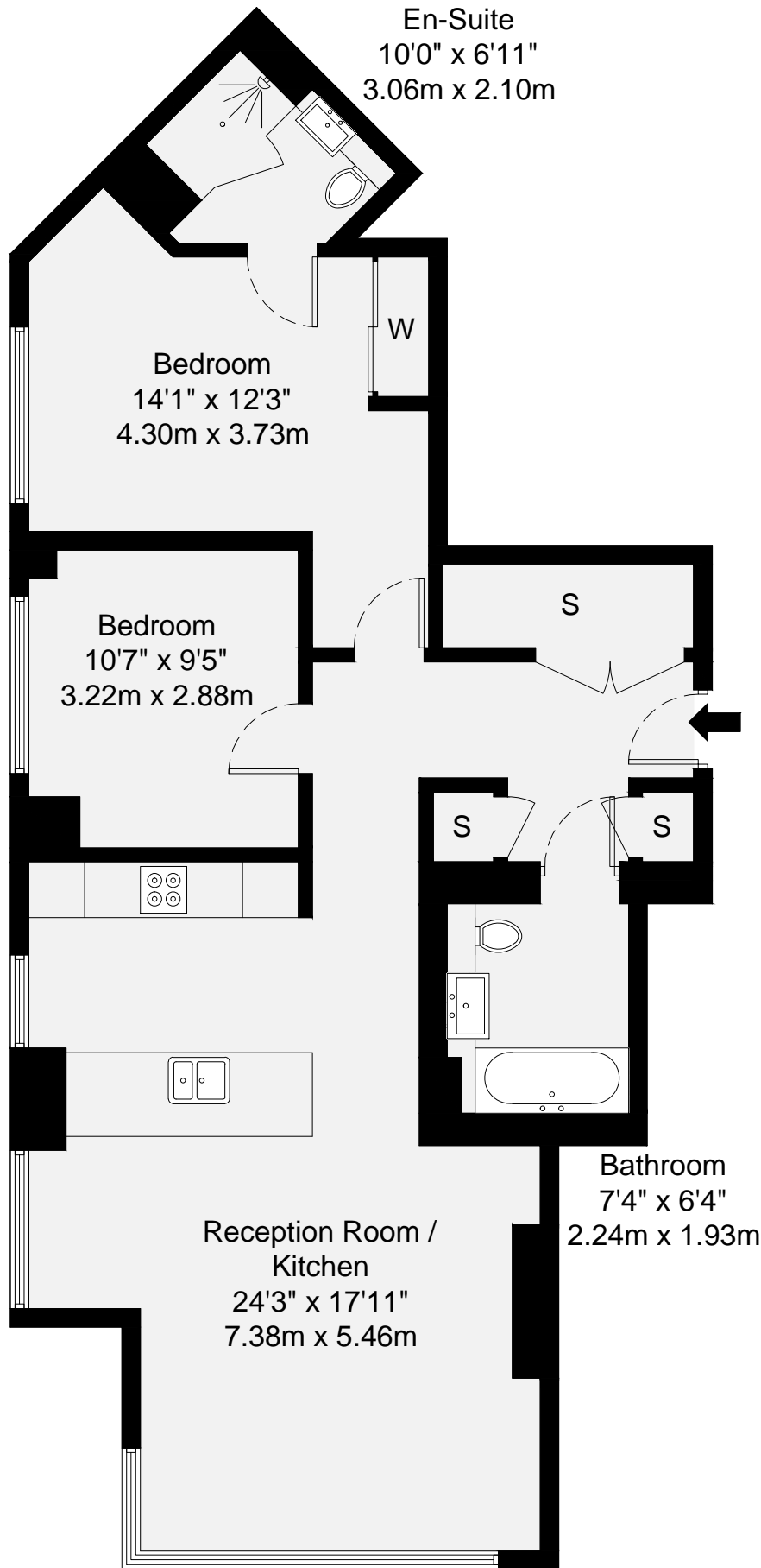
41st Floor
